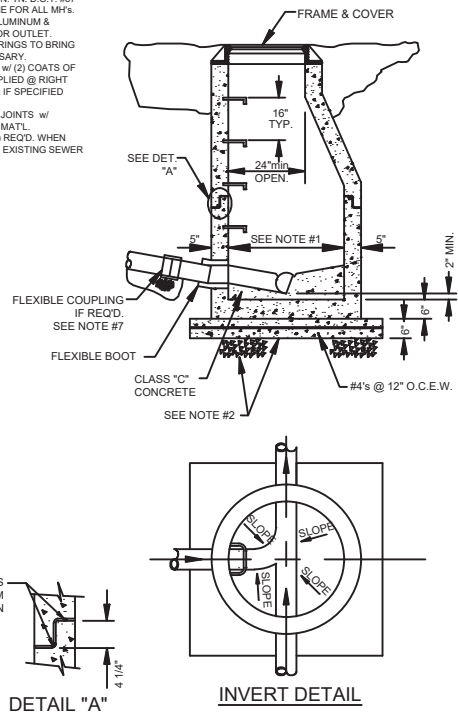
STANDARD PRE-CAST MANHOLE (MH-1) DETAIL
