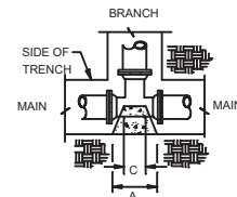
TEE DETAIL
