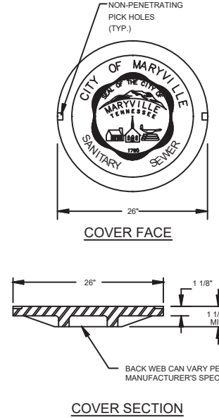
MANHOLE COVER DETAIL
