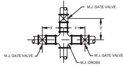
VALVE LOCATIONS @ CROSS
