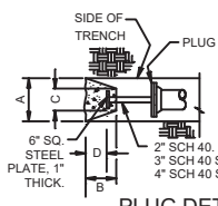
PLUG DETAIL
