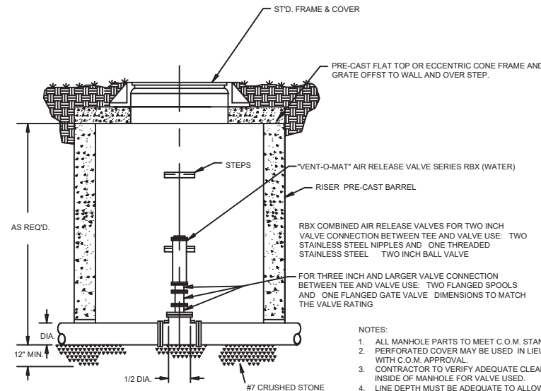
WATER LINE COMBINED AIR RELEASE VALVE
