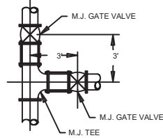
VALVE LOCATIONS @ TEE
