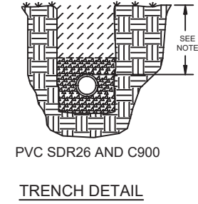
TRENCH DETAIL
