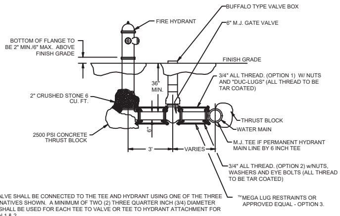
TYPICAL FIRE HYDRANT INSTALLATION
