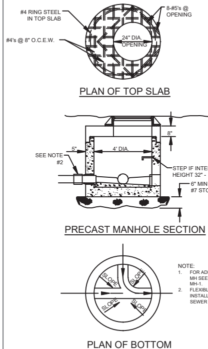
SHALLOW MANHOLE DETAIL
