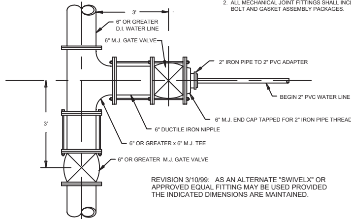
TIE-IN FOR 2" PVC WATER LINE TO 6" OR LARGER MAIN WATER LINE
