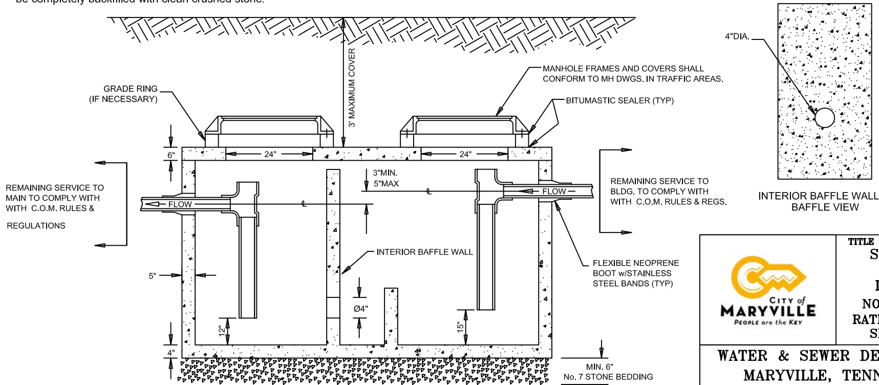
OIL/GRIT SEPERATOR DETAIL (NON-TRAFFIC RATED)
